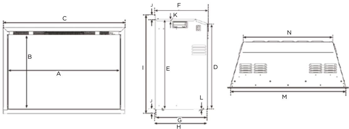
Dimensions (mm)
